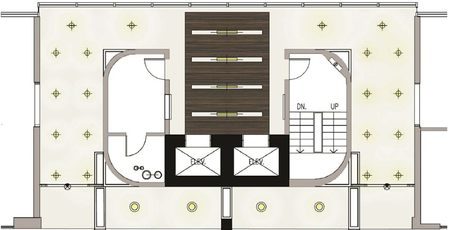
REFLECTED CLG. PLAN OPTION 1
